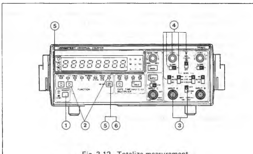
Fig. 3-12 Totalize measurement
