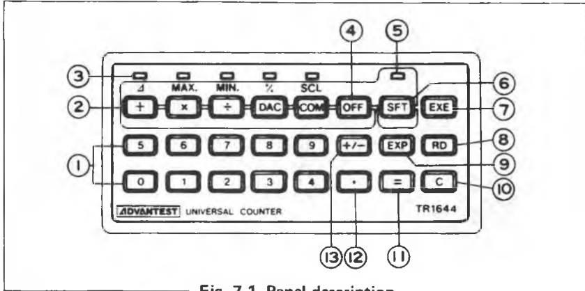
Fig. 7-1 Panel description
