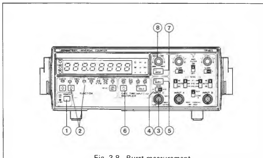
Fig. 3-8 Burst measurement
