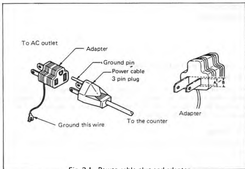
Fig. 3-1 Power cable plug and adapter
