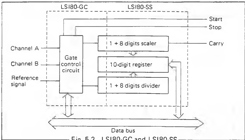
Fig. 5-2 LSI80-GC and LSI80-SS
