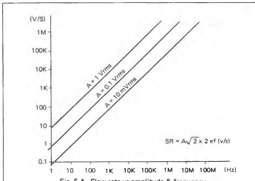
Fig. 5-4 Slew rate vs amplitude & frequency
