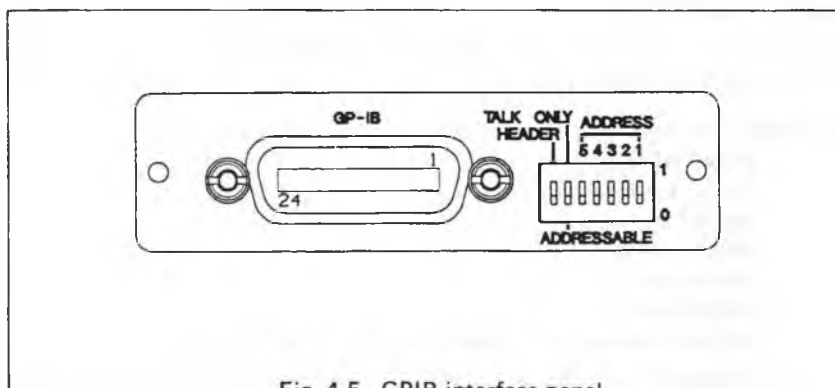
Fig. 4-5 GPIB interface panel
