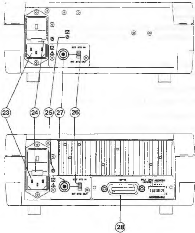
Fig. 3-2 Panel description
