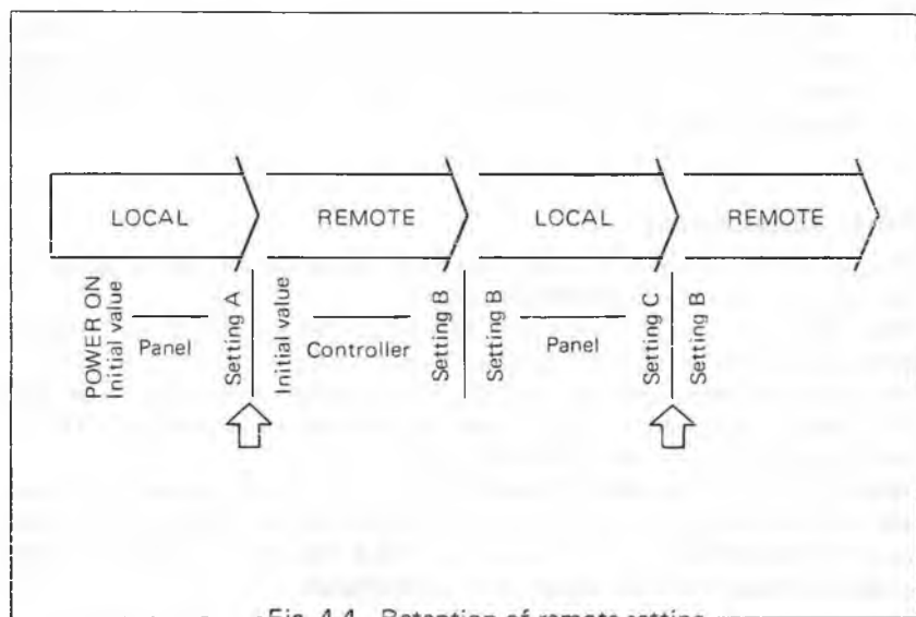
Fig. 4-4 Retention of remote setting
