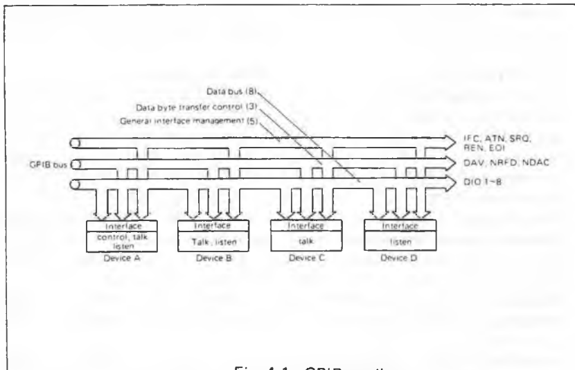
Fig. 4-1 GPIB outline
