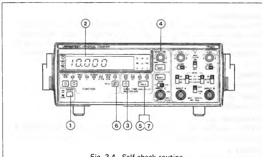
Fig. 3-4 Self-check routine
