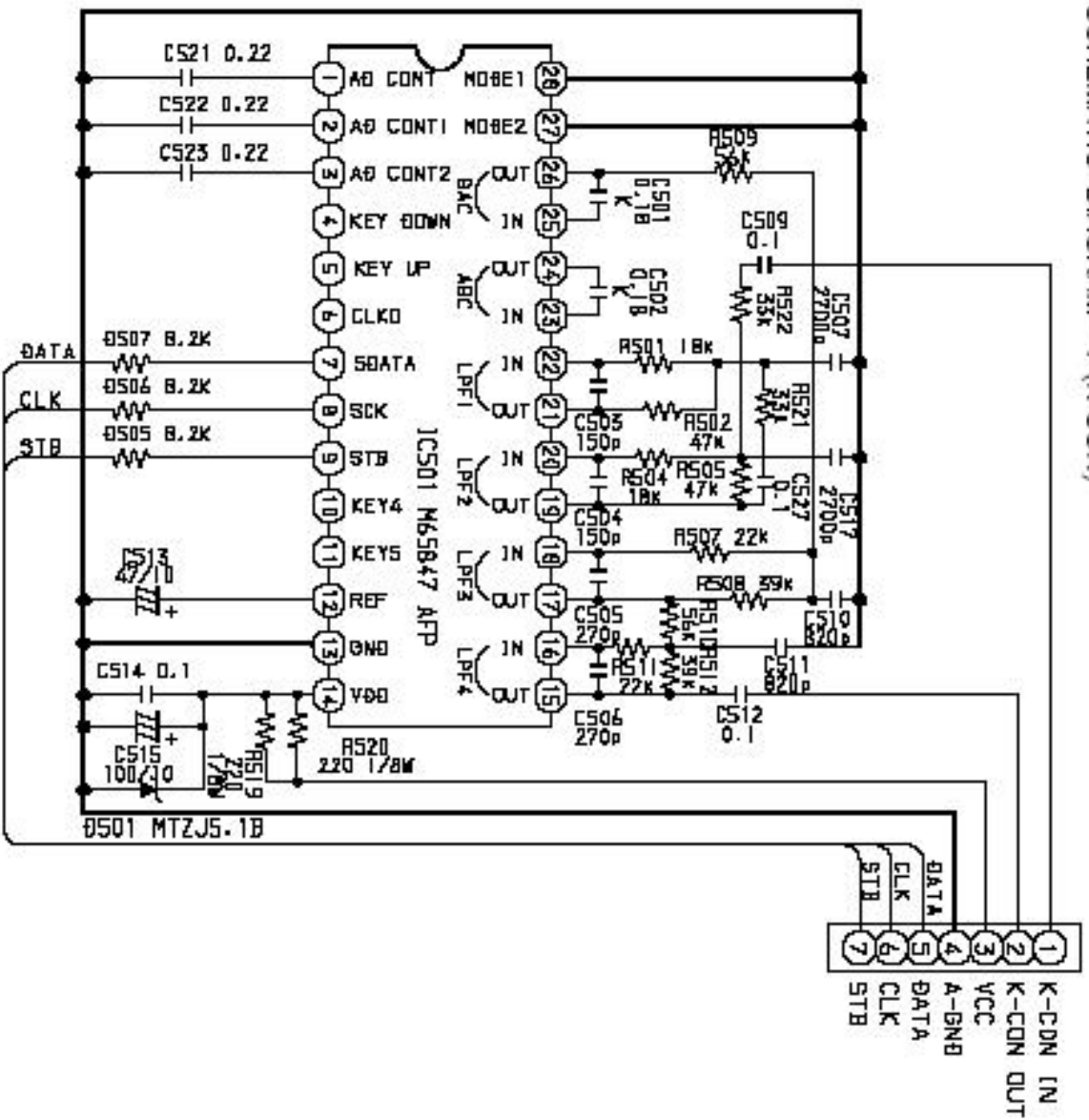
SCHEMATIC DIAGRAM - 7 (K-CON)
