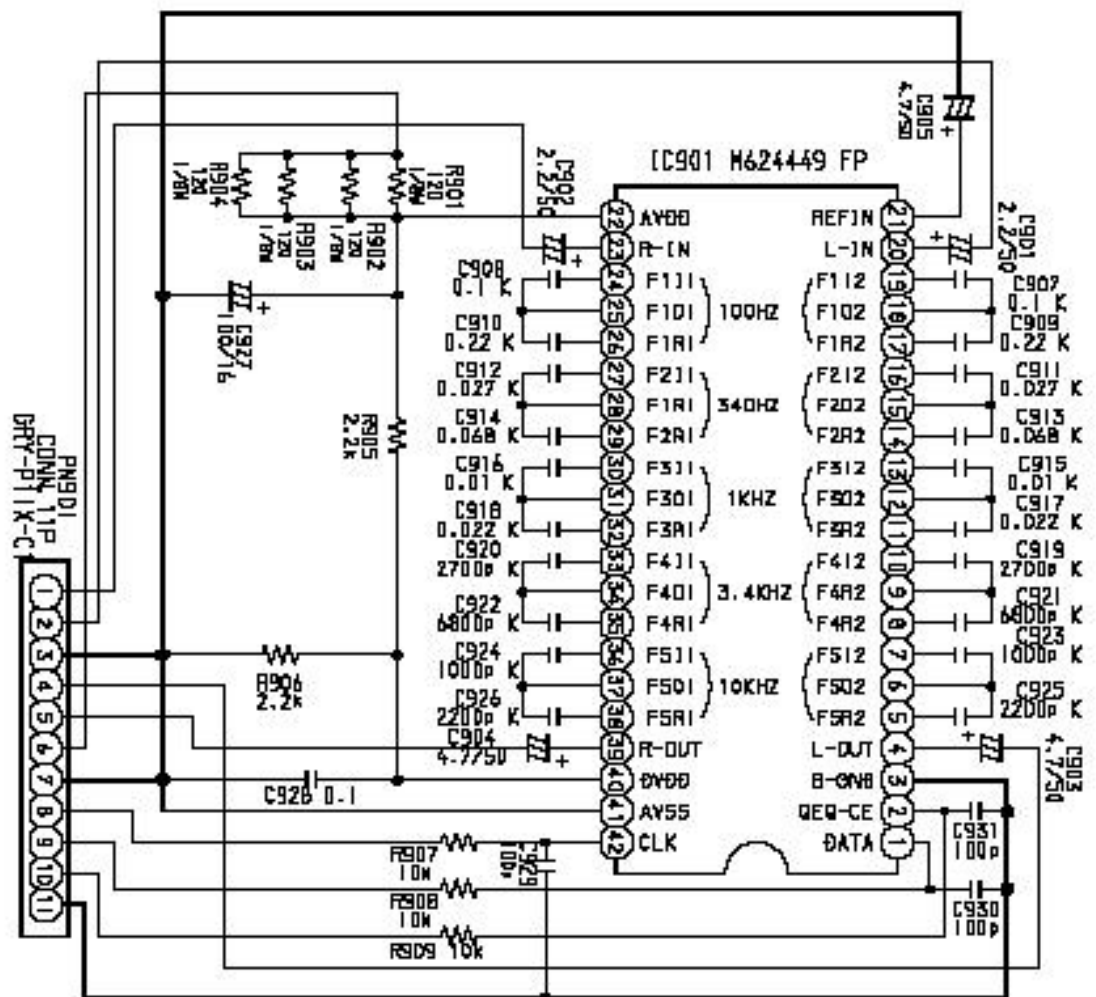
SCHEMATIC DIAGRAM - 6 (GEO)
